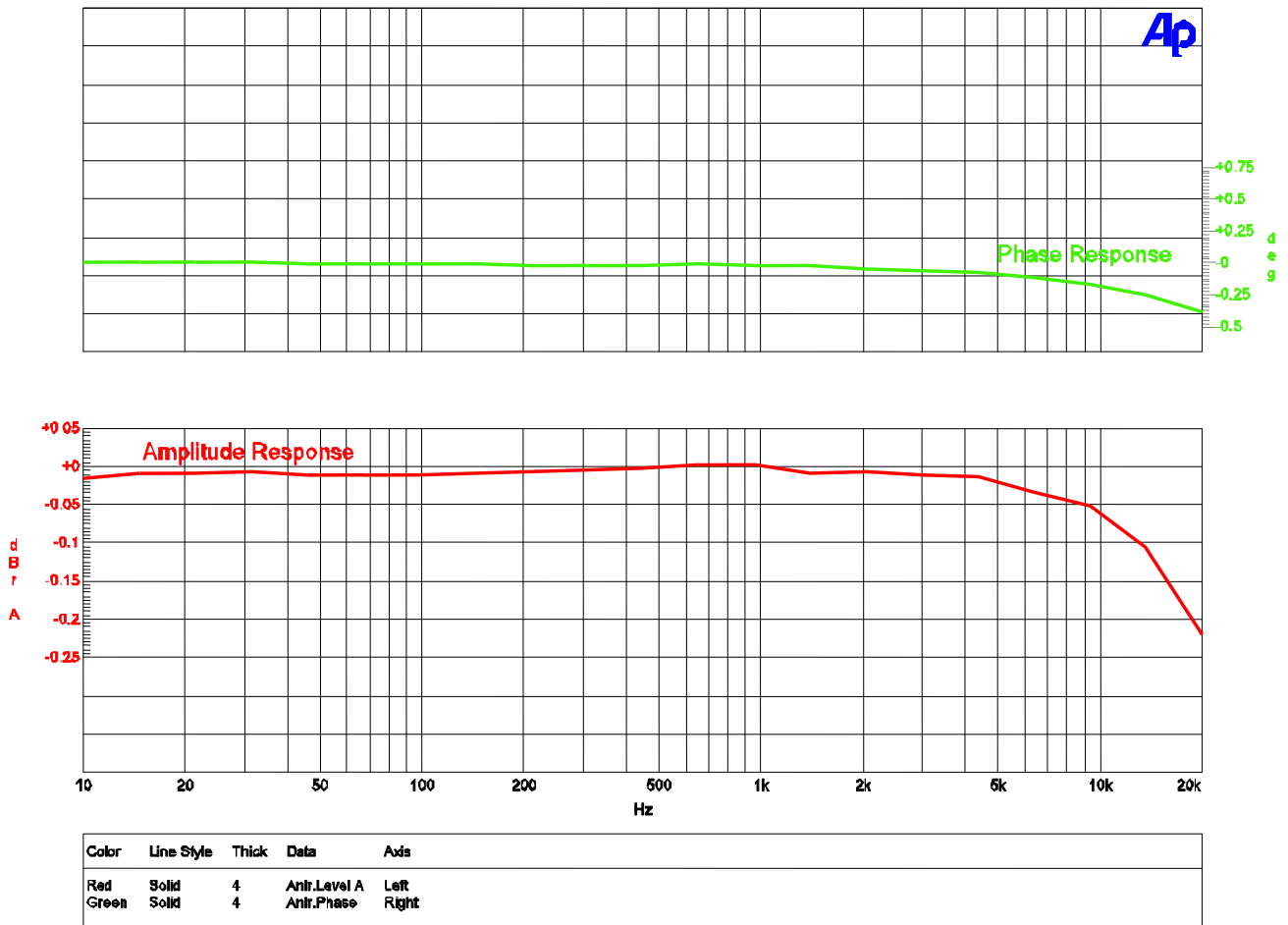
3 - Freq Response.at2c
